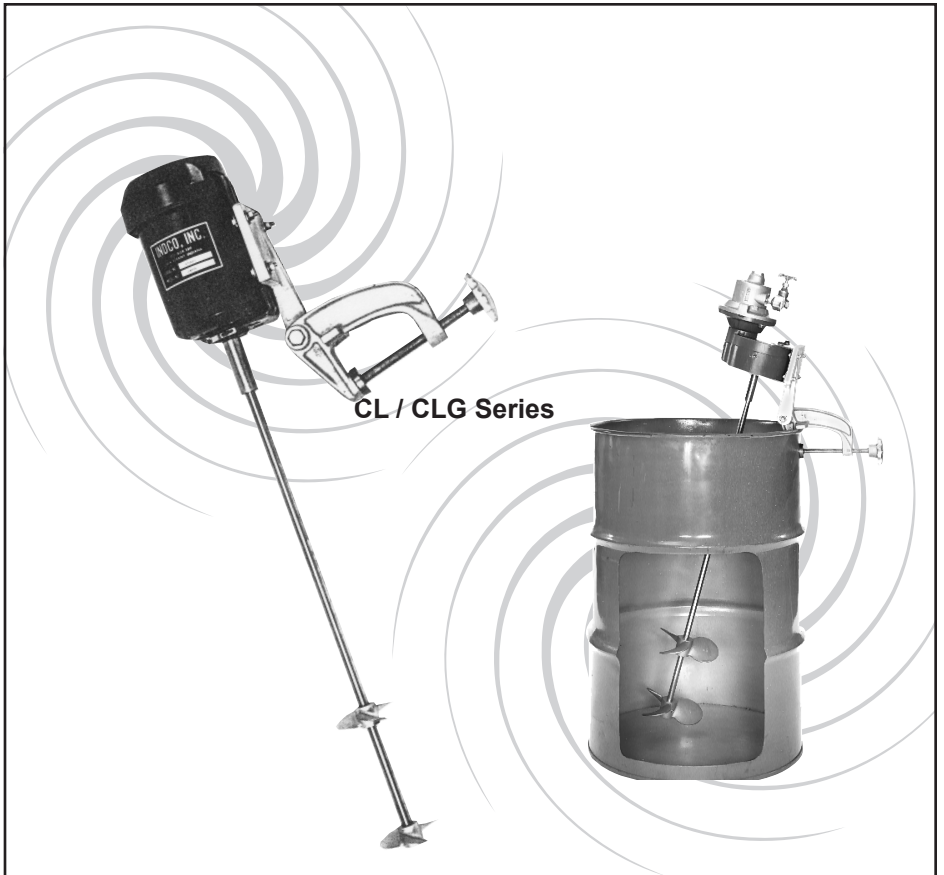
CL / CLG Series CL & CLG SERIES CLAMP MOUNT MIXERS
